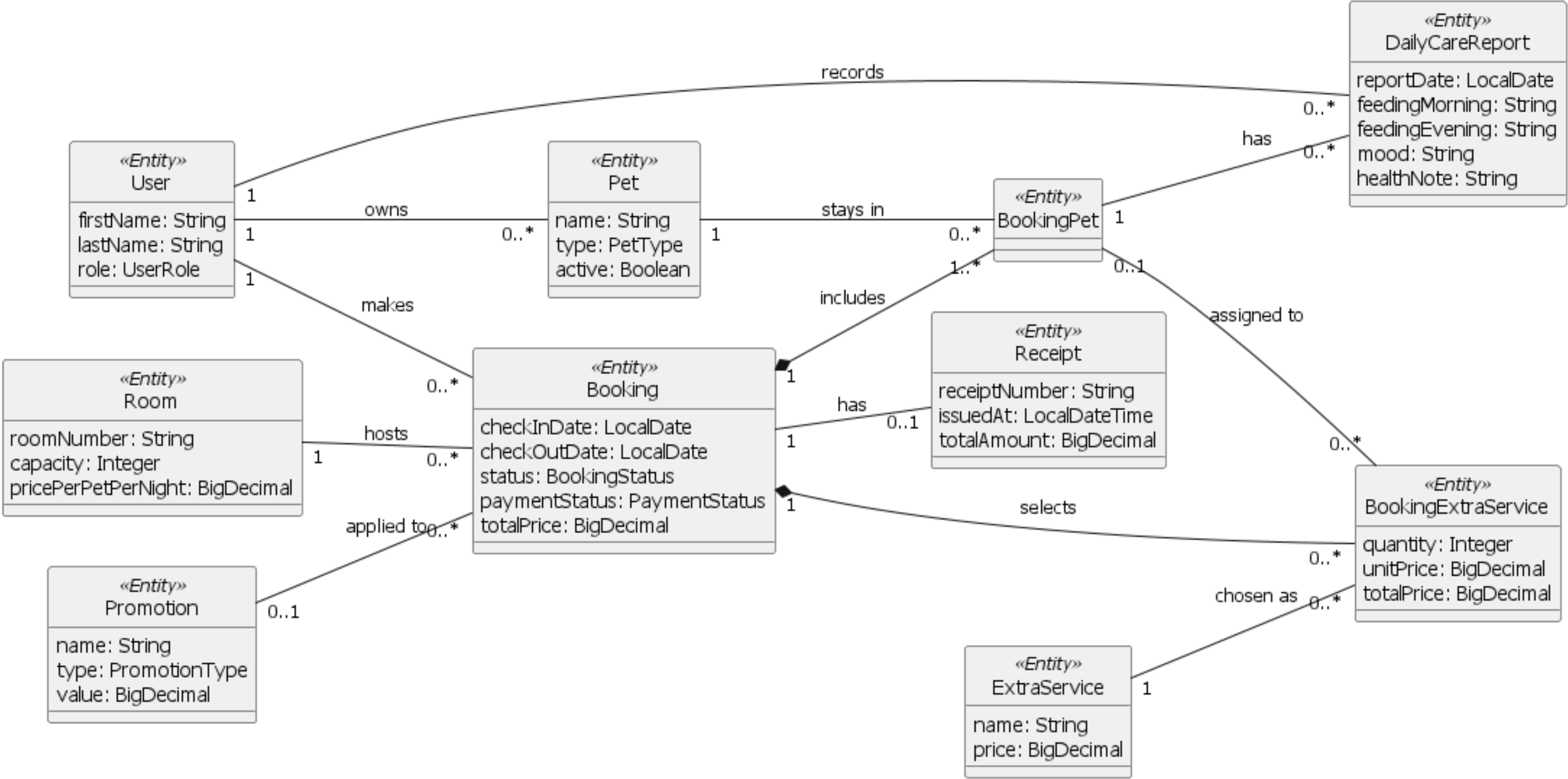
PetsHotel - Domain Model
